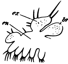
FIG. 209. TYPICAL PHYLLOPOD APPENDAGE. (Copied from Claus.)
